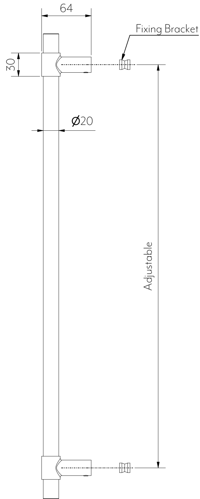
Side View
