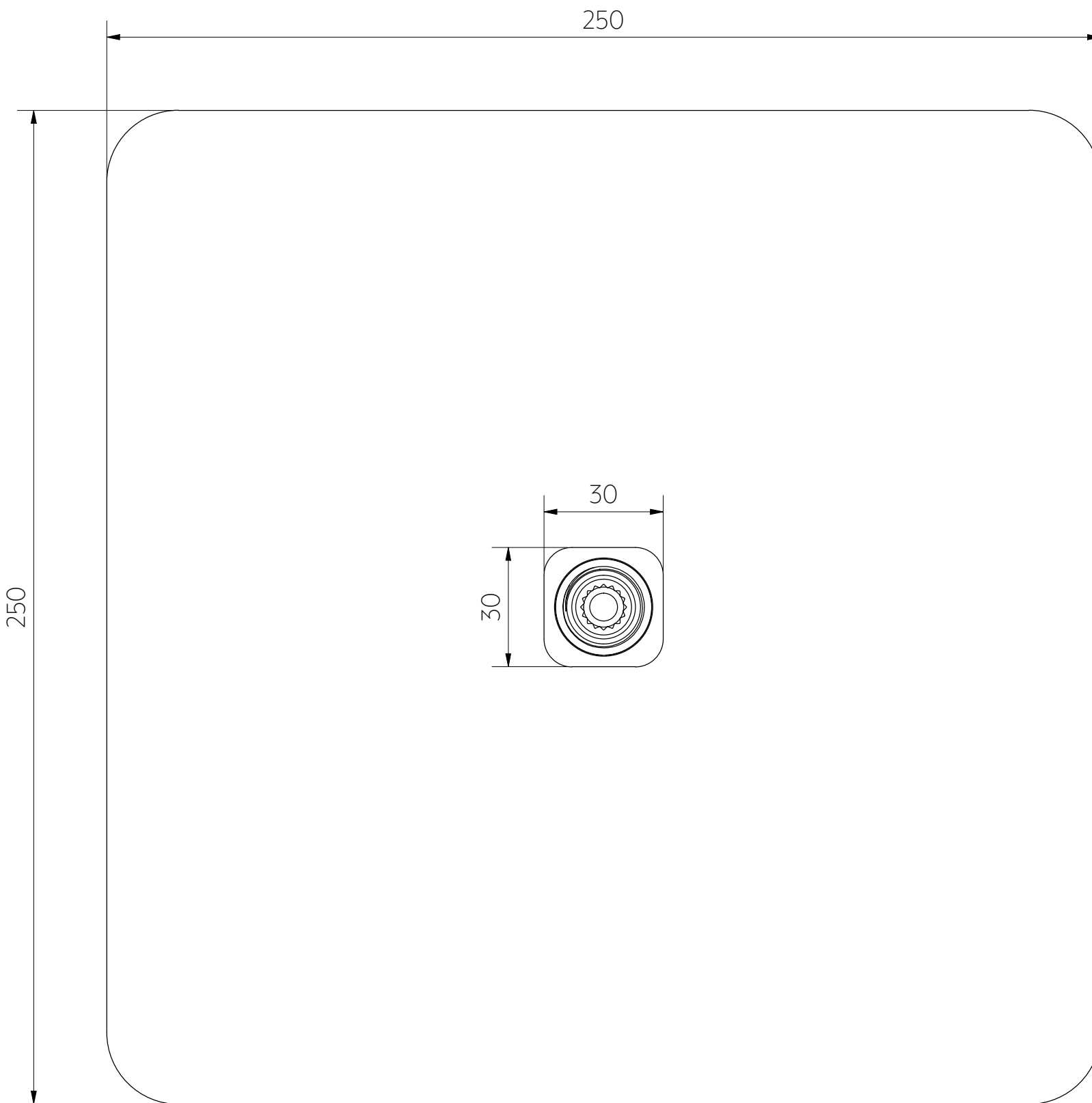
Top View
