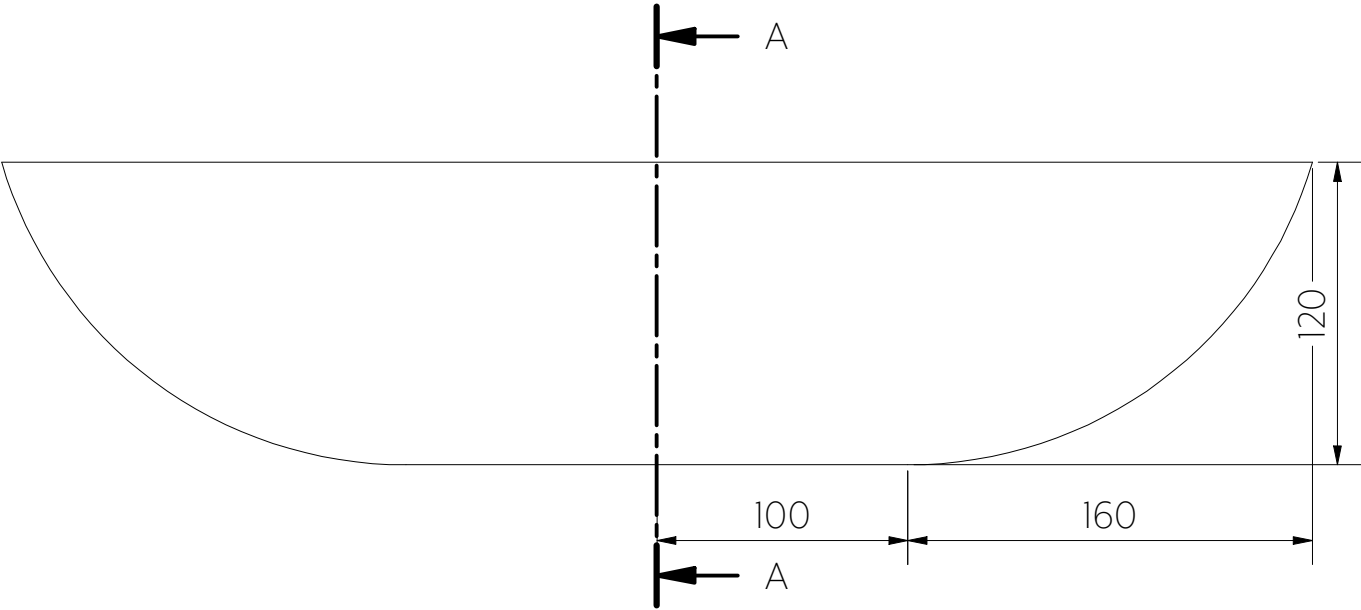
Front View
