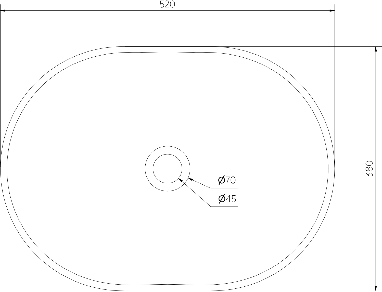
Top View
