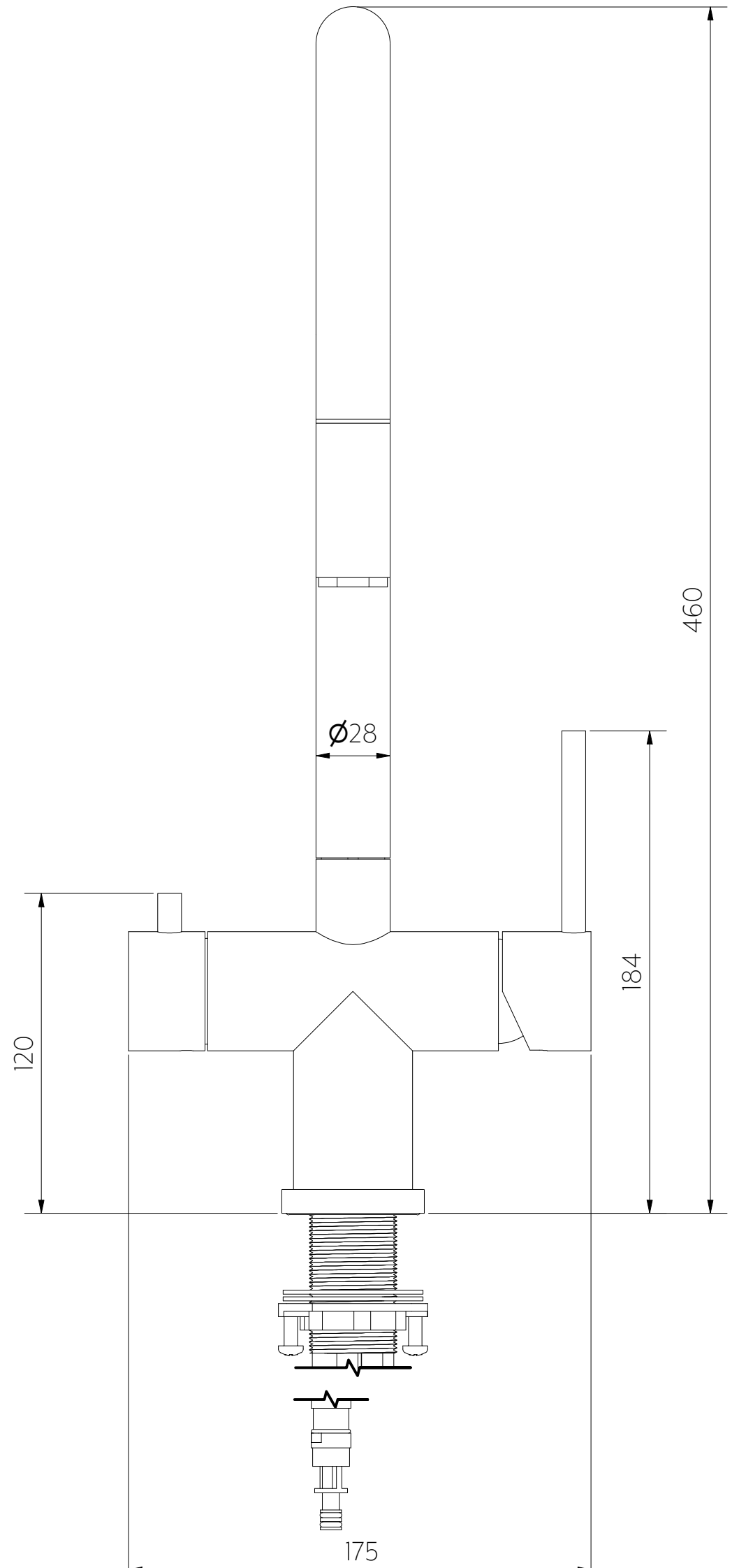
Front View
