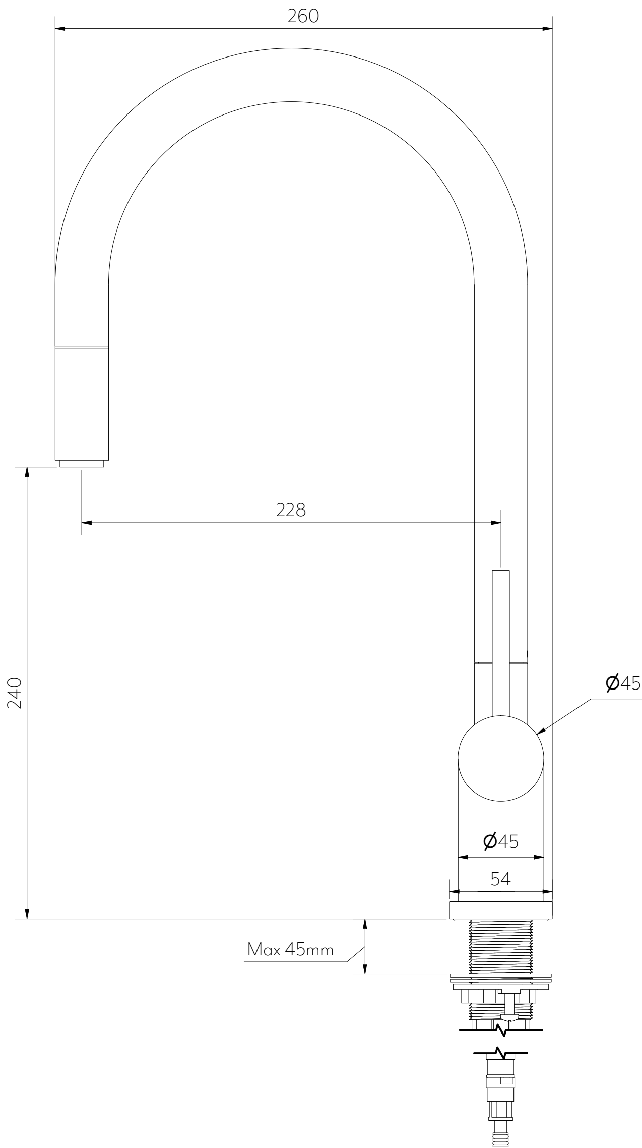
Side View
