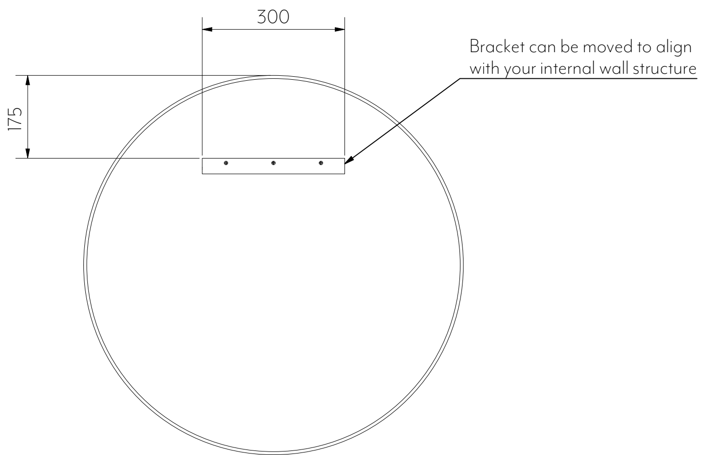
Back View
