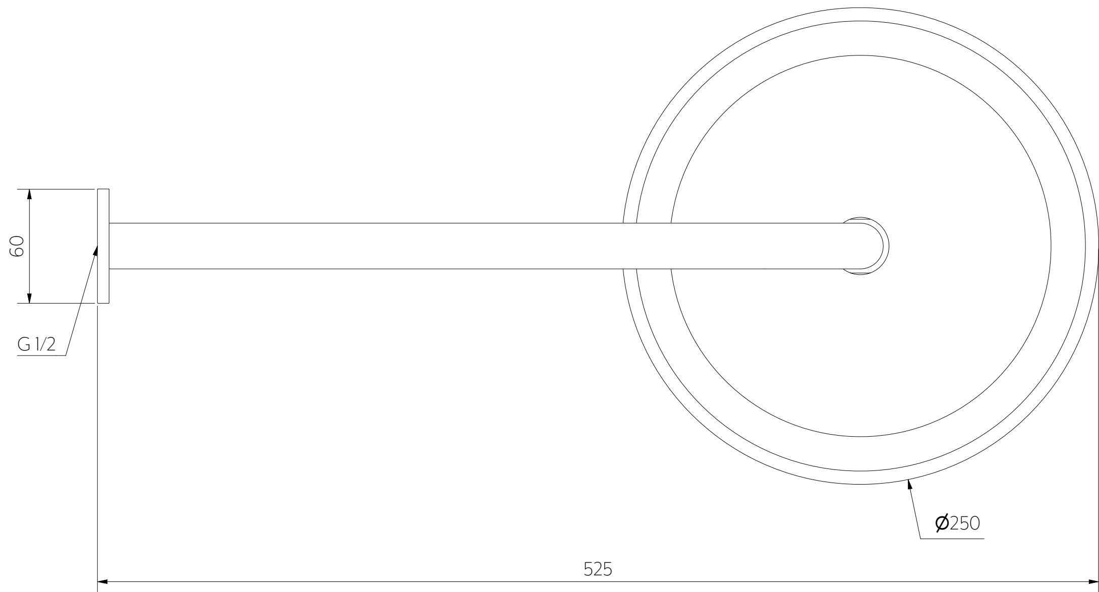
Top View
