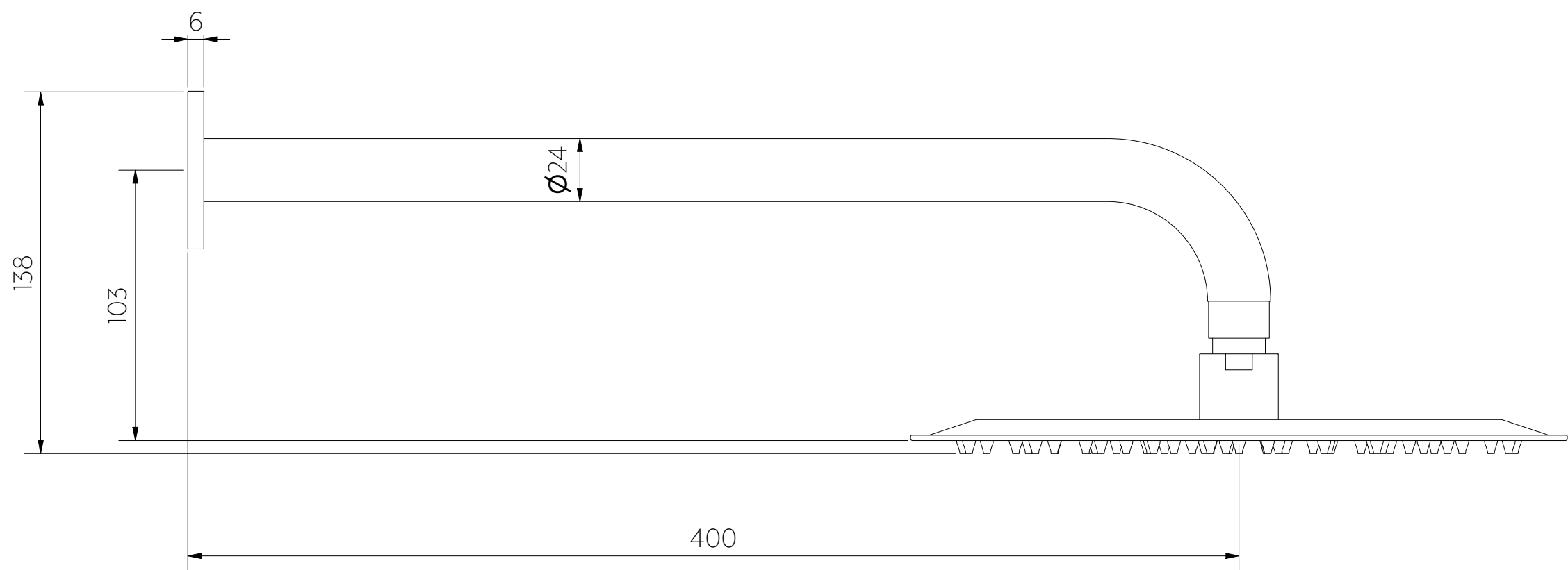
Side View
