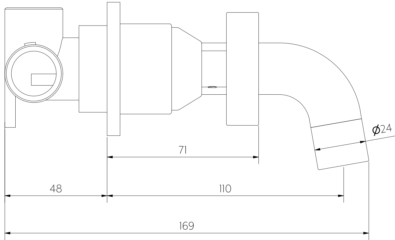
Side View
